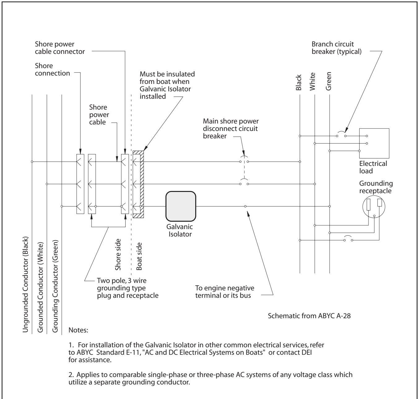
FIGURE 4 Typical Installation of a Galvanic Isolator for Marine Vessel Application
